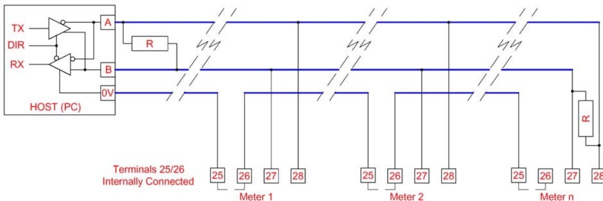
Figure 3-1 Basic RS485 To Internal Modbus Option
